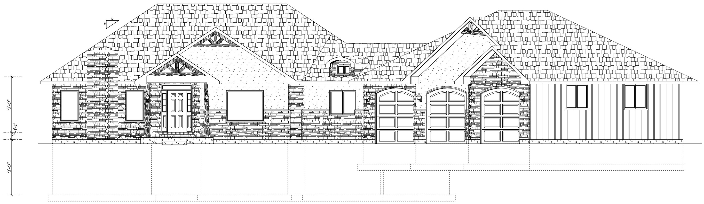
FRONT ELEVATION
