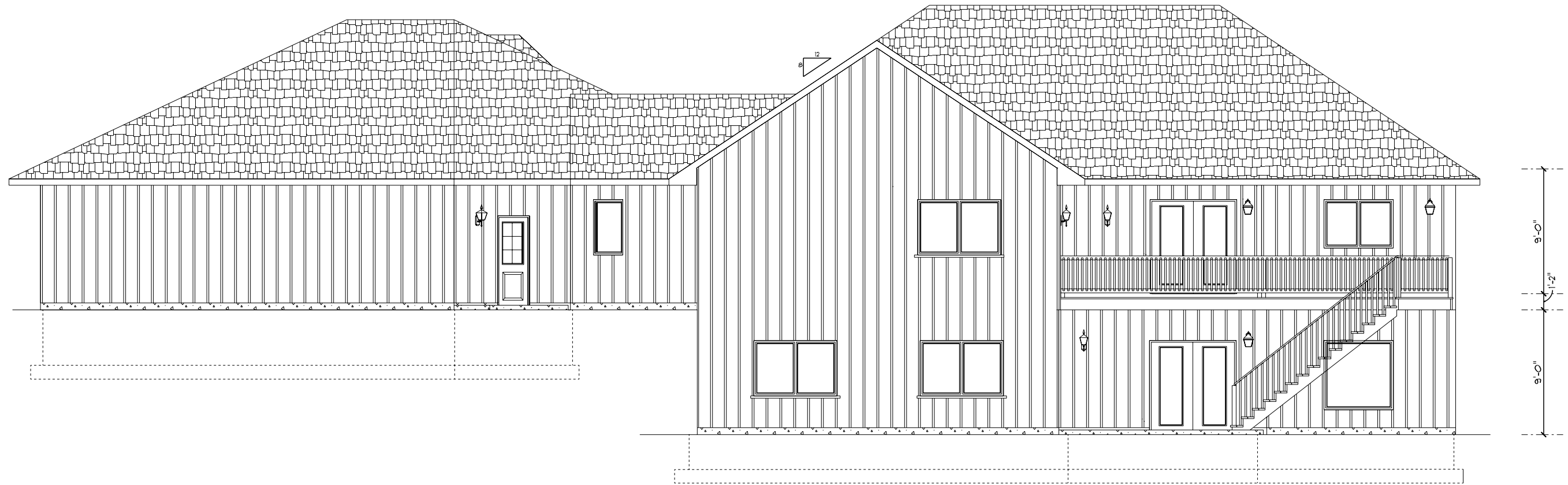
REAR ELEVATION
