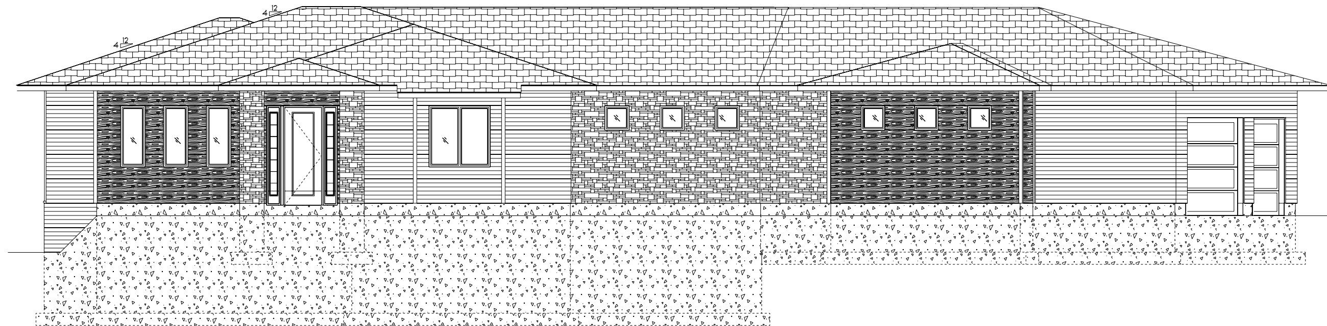
FRONT ELEVATION
