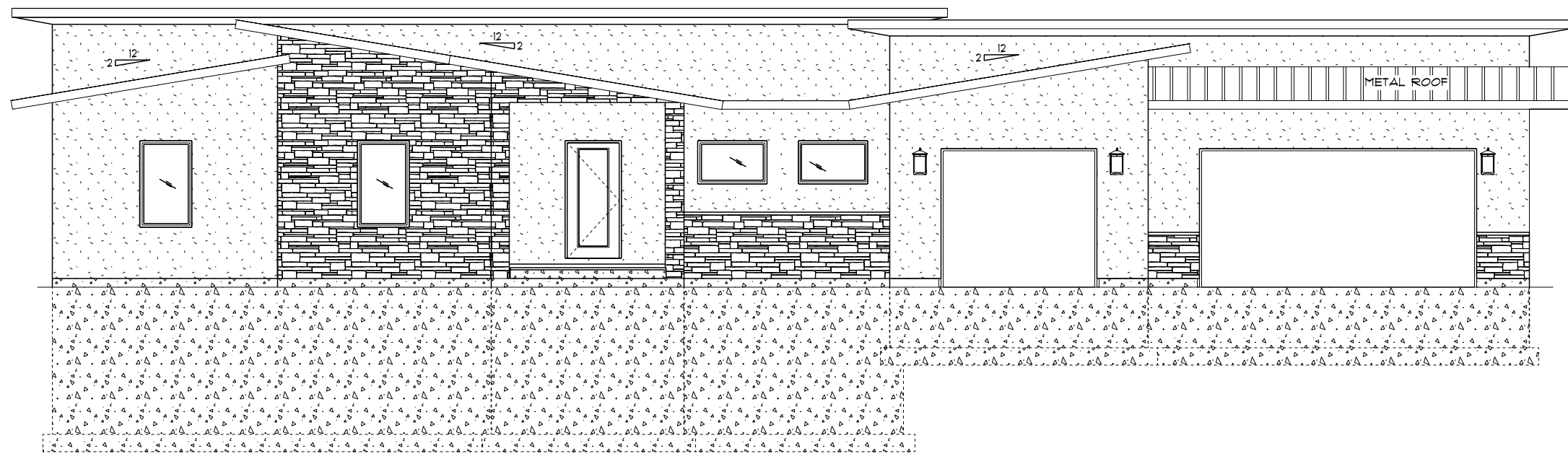
FRONT ELEVATION
